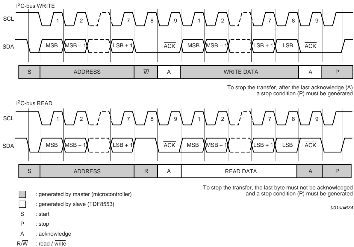
Fig 10. I 2 C-bus read and write modes
