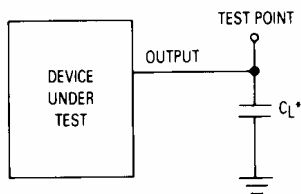
Figure 5. Test Circuit
