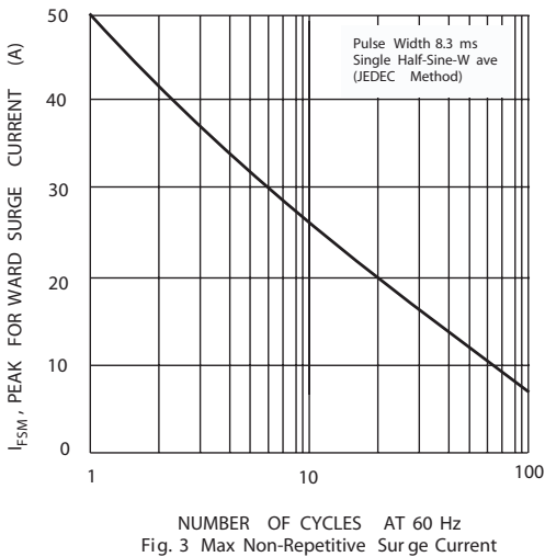
Fig. 3 Max Non-Repetitive Surge Current
