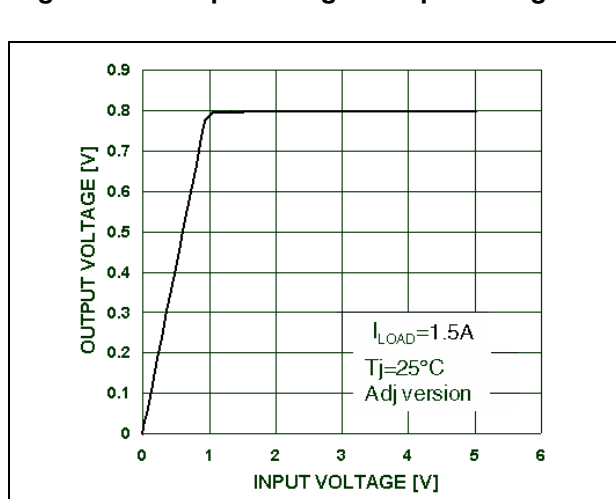
Figure 11. Output voltage vs input voltage
