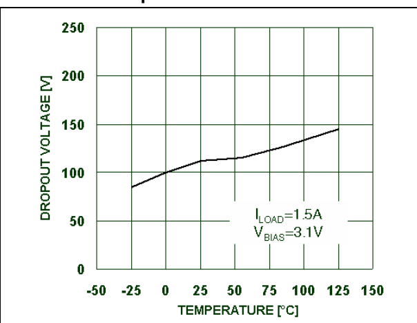
Figure 12. Dropout voltage ( V_{IN}-V_{OUT} ) vs temperature
