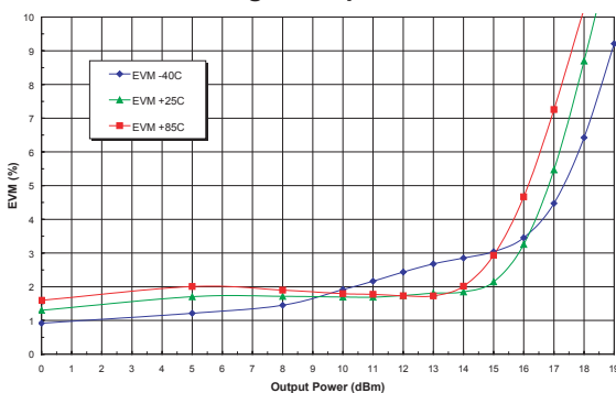
Figure 6: Tx Path EVM vs. Output Power Across Temp (Freq = 2.45 GHz, Vcc = +3.6 V) 802.11g 54 Mbps OFDM
