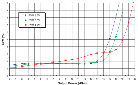
Figure 7: Tx Path EVM vs. Output Power Across Power Supply Voltage (Freq = 2.45 GHz, TA = +25°C) 802.11g 54 Mbps OFDM
