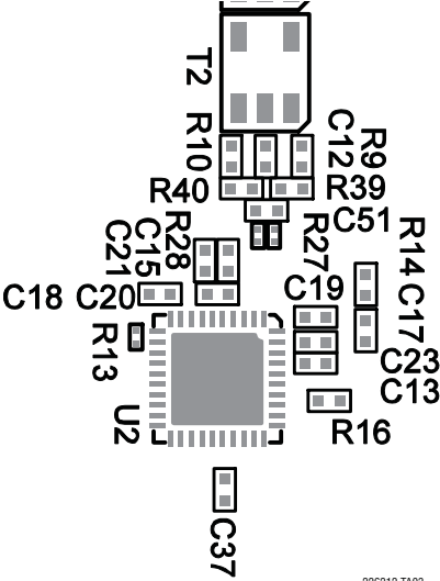
Silkscreen Top
