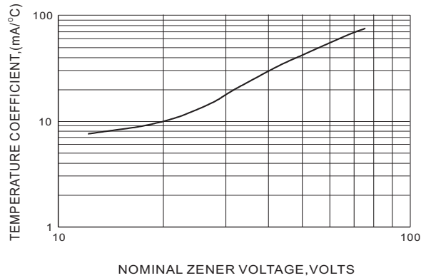
Fig. 2 TEMPERATURE COEFFICIENTS
