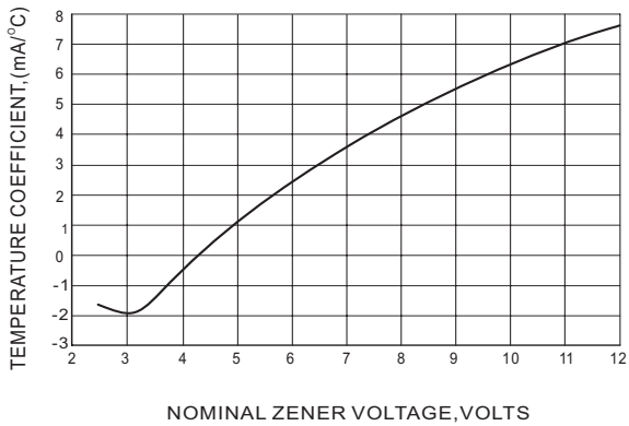
Fig. 1 TEMPERATURE COEFFICIENTS
