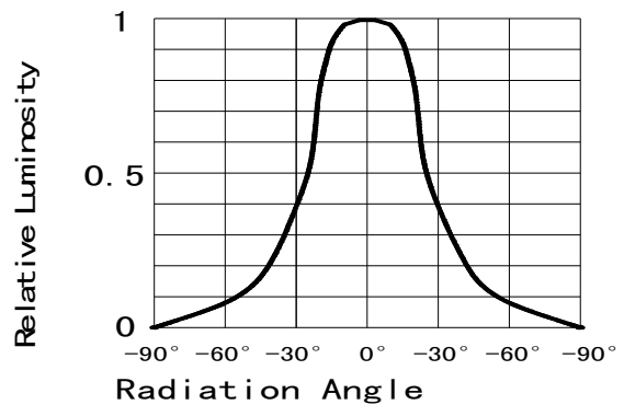
Fig 6. Relative Luminous Intensity vs. Radiation Angle
