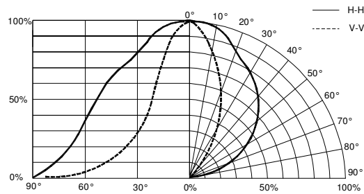
Fig 6. Relative Luminous Intensity vs. Radiation Angle
