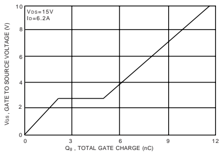
Figure 3. Gate Charge
