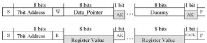
Figure H: Typical I 2 C read transmission. Note: S = START, W = WRITE, R = READ, AK = acknowledged, NACK = NOT acknowledged, P = STOP. Clear boxes originate in the I 2 C Master and shaded boxes originate in the I 2 C Slave.
