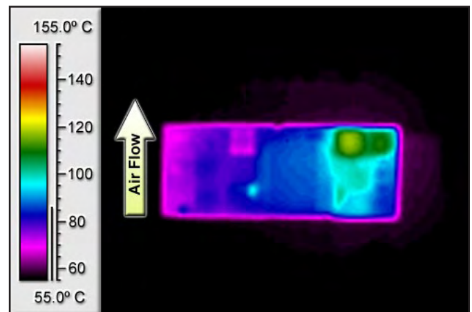
Figure 6: Thermal plot of converter at 17.5 A load current (43.75 W) with 55°C air flowing at the rate of 200 LFM. Air is flowing across the converter from pin 3 to pin 1 (nominal input voltage).
