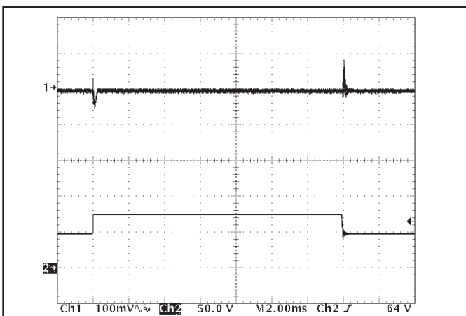
Figure 17: Output voltage response to step-change in input voltage ( 48\ \text{V} to 75\ \text{V} ), at 20\ \text{A} load current. Load cap: 15\ \mu\text{F} tantalum capacitor and 1\ \mu\text{F} ceramic cap. Ch 1: V_{OUT} ( 100\ \text{mV}/\text{div} ), Ch 2: V_{IN} ( 50\ \text{V}/\text{div} ).
