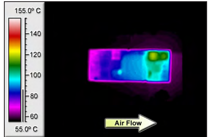
Figure 8: Thermal plot of converter at 18.6 A load current (42W) with 55°C air flowing at the rate of 200 LFM. Air is flowing across the converter from input to output (nominal input voltage).
