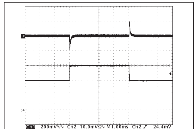
Figure 12: Output voltage response to step-change in load current (50%-75%-50% of I out (max); di/dt = 1A/ \mu s). Load cap: 470 \mu F, 30 m \Omega ESR tantalum cap and 1 \mu F ceramic cap. Ch 1: V out (200mV/div), Ch 2: I out (5A/div).
