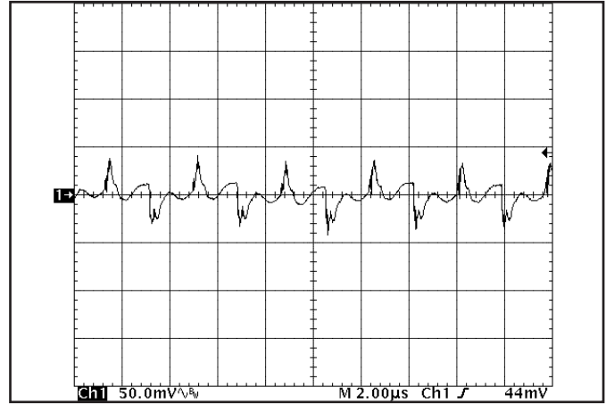
Figure 20: Output voltage ripple at nominal input voltage and rated load current (50 mV/div). Load capacitance: 1 \mu\text{F} ceramic capacitor and 10 \mu\text{F} tantalum capacitor. Bandwidth: 500 MHz. See Figure 17.
