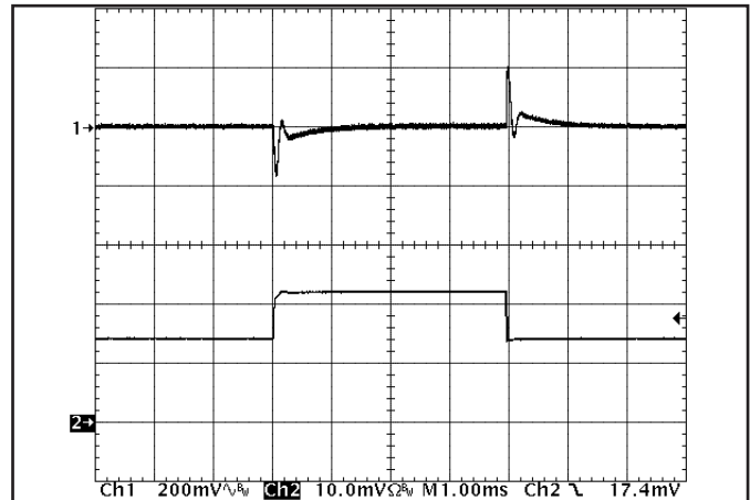
Figure 16: Output voltage response to step-change in load current (50%-75%-50% of I_{out(max)} ; di/dt = 1A/\mu s ). Load cap: 470\mu F , 30\text{ m}\Omega ESR tantalum cap and 1\mu F ceramic cap. Ch 1: V_{out} (200mV/div), Ch 2: I_{out} (20A/div).
