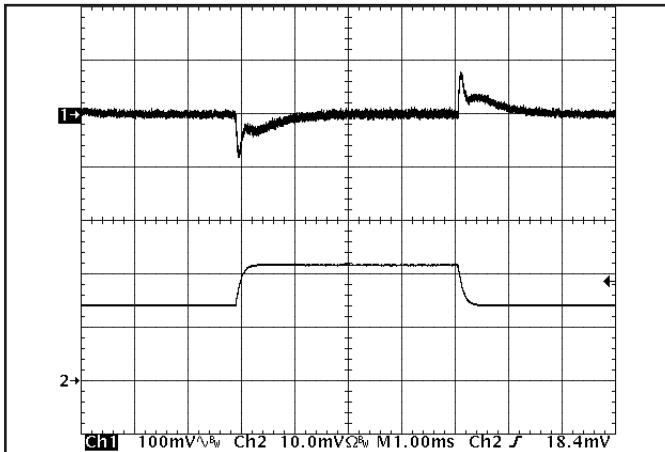
Figure 15: Output voltage response to step-change in load current (50%-75%-50% of I_{out(max)} ; di/dt = 0.1A/\mu s ). Load cap: 10\mu F , 100\text{ m}\Omega ESR tantalum cap and 1\mu F ceramic cap. Ch 1: V_{out} (100mV/div), Ch 2: I_{out} (20A/div).
