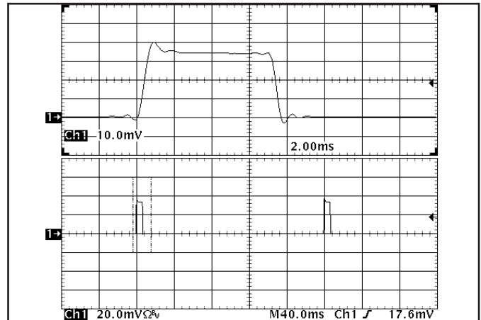
Figure 22: Load current (20A/div) as a function of time when the converter attempts to turn on into a 1 \text{ m}\Omega short circuit. Top trace (2ms/div) is an expansion of the on-time portion of the bottom trace.
