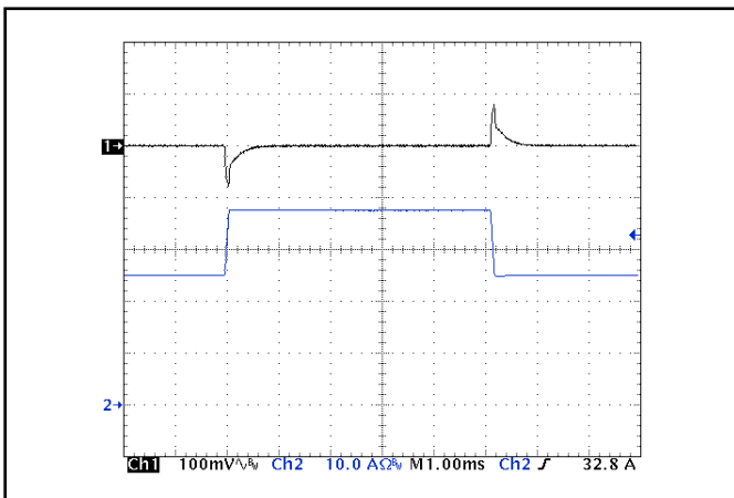
Figure 5: Output voltage response to step-change in load current (50%-75%-50% of I out (max); dI/dt = 0.2 A/μs). Load cap: 1 μF ceramic and 15 μF tantalum capacitors. Ch 1: V out (100 mV/div), Ch 2: I out (10 A/div).
