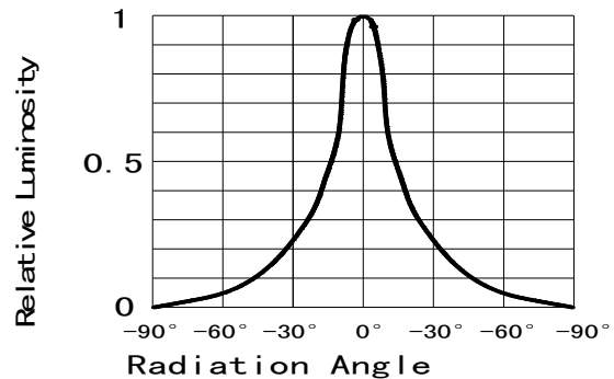
Fig 6. Relative Luminous Intensity vs. Radiation Angle
