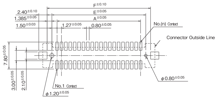
PCB Mounting Dimensions (View from Mounting Side)
