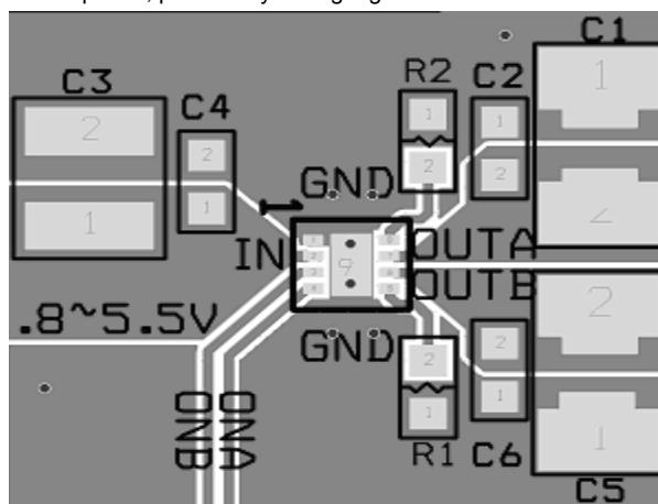
Figure 39. Proper Layout of Output and Ground Copper Area
