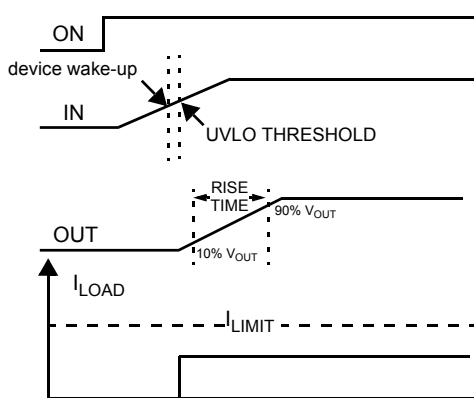
Figure 36. Under-Voltage Lockout (UVLO)
