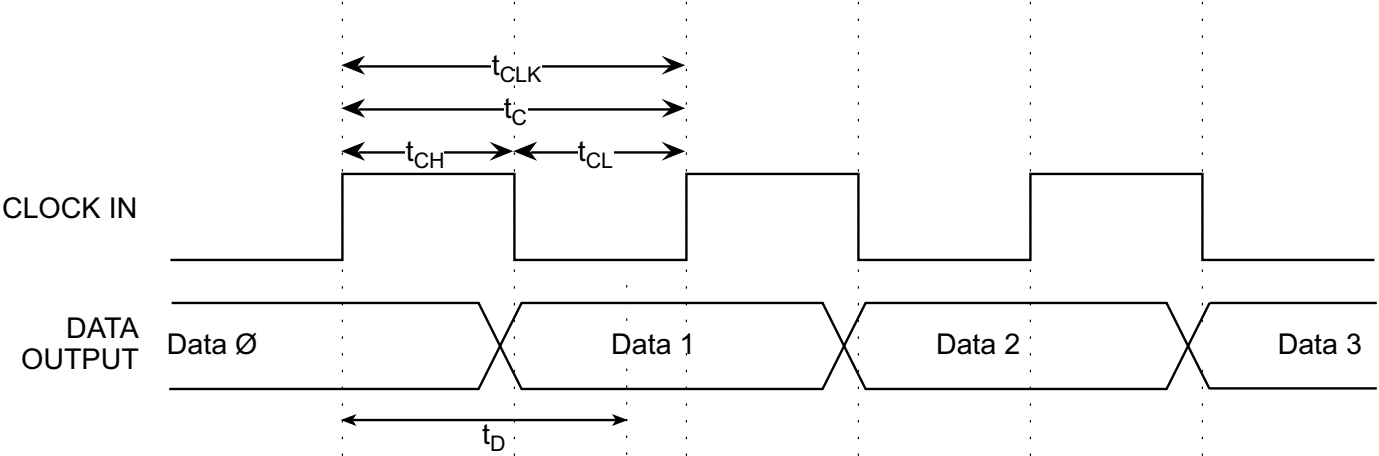
Figure 1b – Timing Diagram
