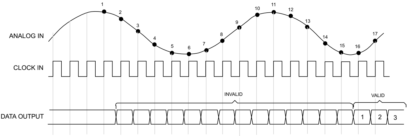
Figure 1a – Timing Diagram
