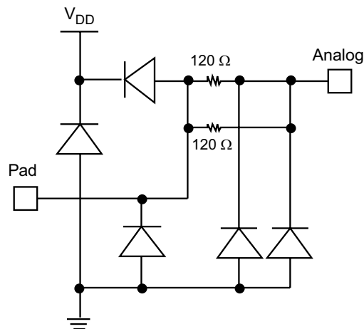
Figure 6 – On-Chip Protection Circuit
