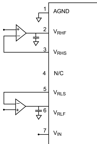
Figure 3 – Ladder Force/Sense Circuit
