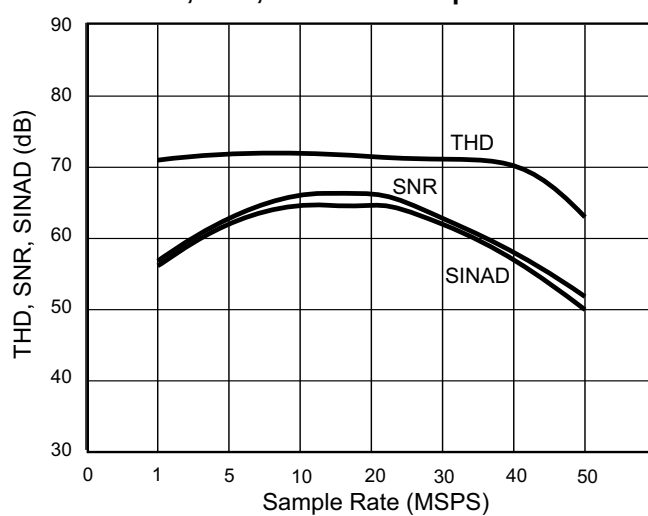
THD, SNR, SINAD vs Sample Rate
