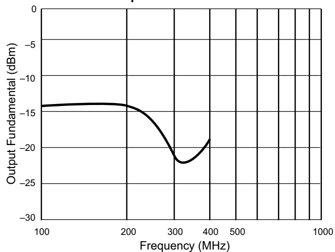
Input Bandwidth
