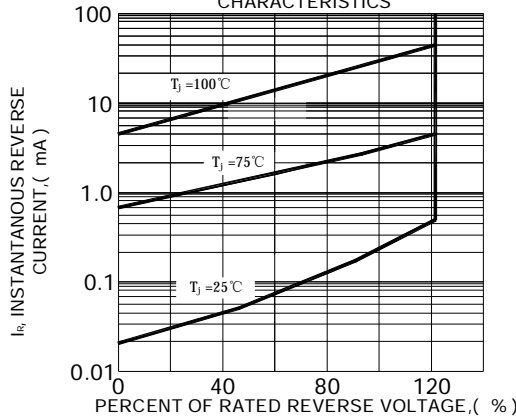
FIG.5-TYPICAL REVERSE CHARACTERISTICS
