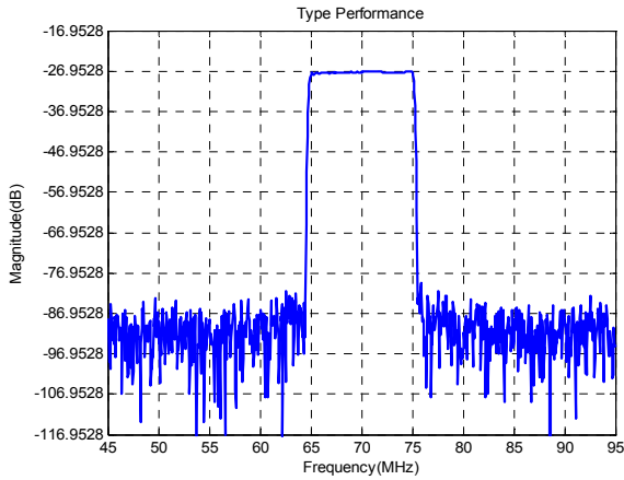
Frequency Respond
