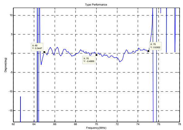
Phase Linearity(f0±MHz)
