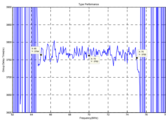
Group Delay Variation(f0±MHz)
