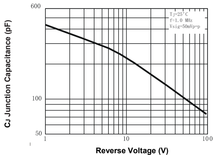
Fig.5-Typical junction capacitance
