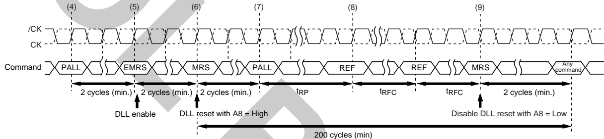
Power-up Sequence after CKE Goes High
