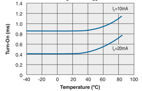
Typical Turn-On vs. Temperature ( I_L=100mA_{DC} )
