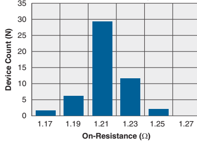
Typical On-Resistance Distribution (N=50, T_A=25^\circ\text{C} , I_L=0.7A_{DC} , I_F=10\text{mA} )
