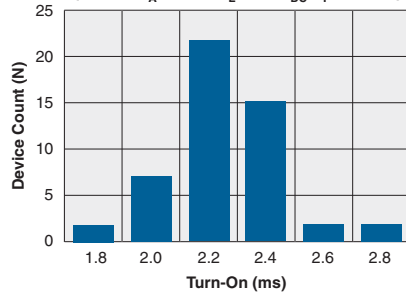
Typical Turn-On Time (N=50, T_A=25^\circ\text{C} , I_L=5mA_{DC} , I_F=10\text{mA} )
