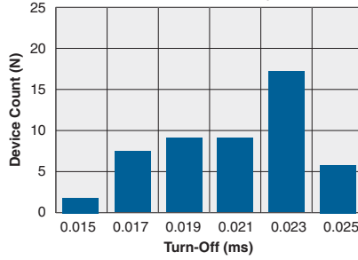
Typical Turn-Off Time (N=50, T_A=25^\circ\text{C} , I_L=5mA_{DC} , I_F=10\text{mA} )
