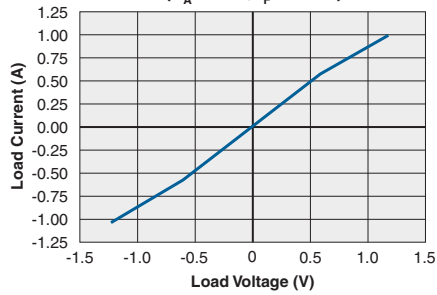
Typical Load Current vs. Load Voltage ( T_A=25^\circ\text{C} , I_F=10\text{mA} )
