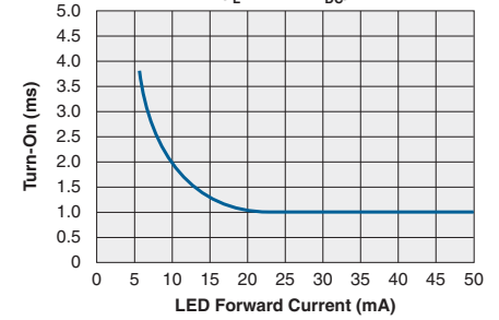
Typical Turn-On vs. LED Forward Current ( I_L=100mA_{DC} )
