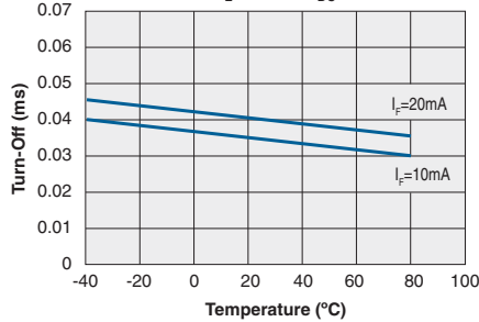
Typical Turn-Off vs. Temperature ( I_L=100mA_{DC} )
