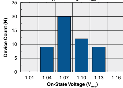
Typical On-State Voltage ( T_A=25^\circ\text{C} , I_L=1\text{A}_{\text{rms}} )
