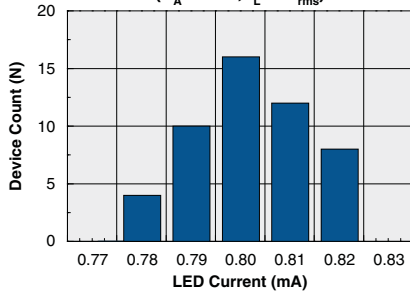
Typical I_F for Switch Operation ( T_A=25^\circ\text{C} , I_L=1\text{A}_{\text{rms}} )
