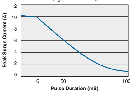
Maximum Surge Current (non-repetitive) ( T_J=50^\circ\text{C max} )
