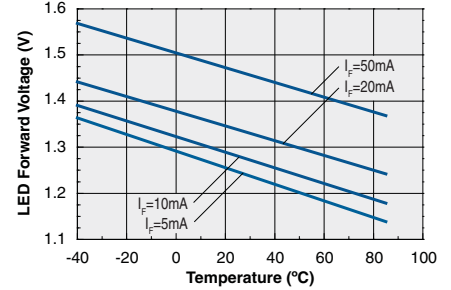
Typical LED Forward Voltage vs. Temperature
