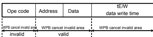
Fig.45 WPB valid timing (WRITE)
