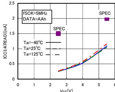
Fig.13 Consumption Current at READ operation ICC_{3,4}
