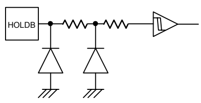
Fig.59 HOLDB input equivalent circuit
