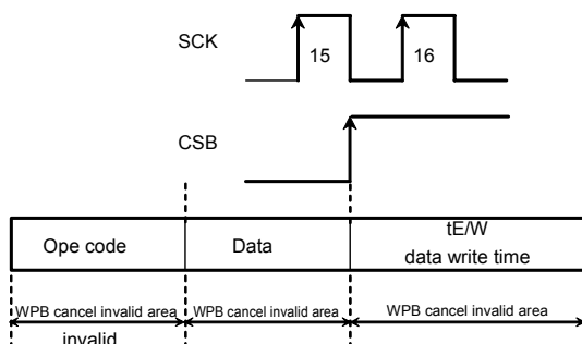
Fig.44 WPB valid timing (WRSR)
