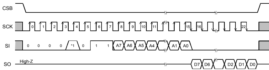
Fig.35 Read command (BR25H010/020/040-W) *1 BR25H010/020-W=Don't care BR25H040-W=A8
