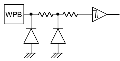
Fig.60 WPB input equivalent circuit
