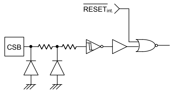
Fig.56 CSB input equivalent circuit
