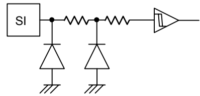
Fig.58 SI input equivalent circuit
