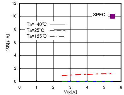
Fig.14 Consumption current at standby operation ISB
