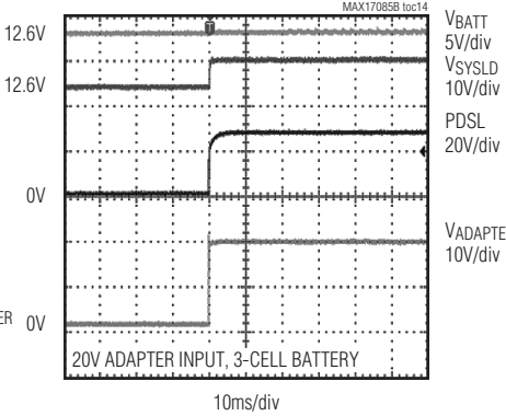
POWER-SOURCE SELECTOR SCHEME WHEN BATTERY IS PRESENT (ADAPTER INSERTION)
