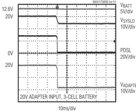
POWER-SOURCE SELECTOR SCHEME WHEN BATTERY IS PRESENT (ADAPTER REMOVAL)
