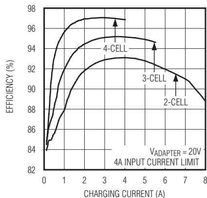
CHARGER EFFICIENCY vs. CHARGING CURRENT
