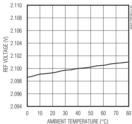
V_{REF} vs. AMBIENT TEMPERATURE
