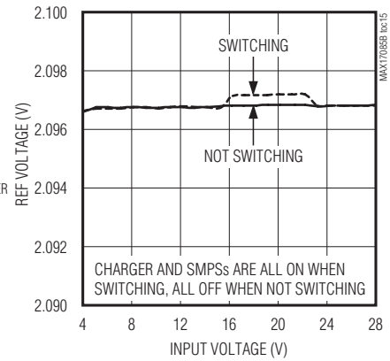
V_{REF} LINE REGULATION (SWITCHING AND NOT SWITCHING)
