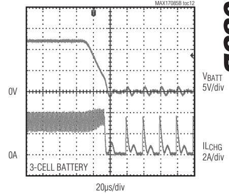
CHARGER OUTPUT SHORT CIRCUIT
