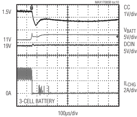
POWER-SOURCE SELECTOR SCHEME WHEN BATTERY IS PRESENT (ADAPTER REMOVAL)
