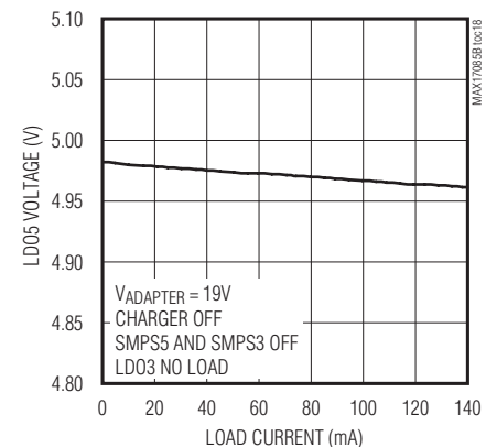
LDO5 LOAD REGULATION
