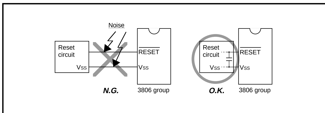
Fig. 3.4.1 Wiring for the RESET pin
