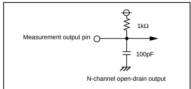
Fig. 3.1.2 Circuit for measuring output switching characteristics (2)
