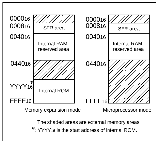
Fig. 37 Memory maps in various processor modes
