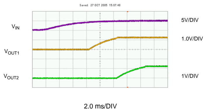
Figure 6: Startup with Sequencing and Soft Start ( C_{OUT} = 22 \mu F)
