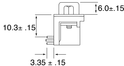
Dimension - mm (Female)
