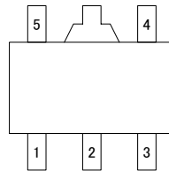
SOT-89-5 (TOP VIEW)
