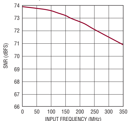
LTC2172-14: SNR vs Input Frequency, -1dBFS, 2V Range, 65Mps
