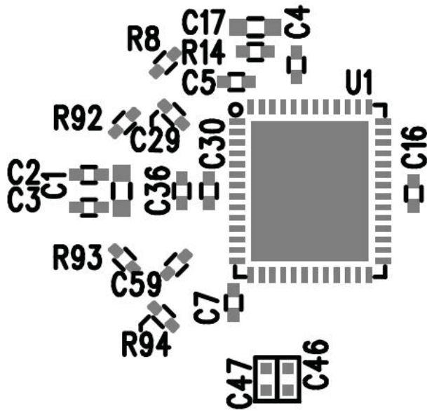
Silkscreen Top
