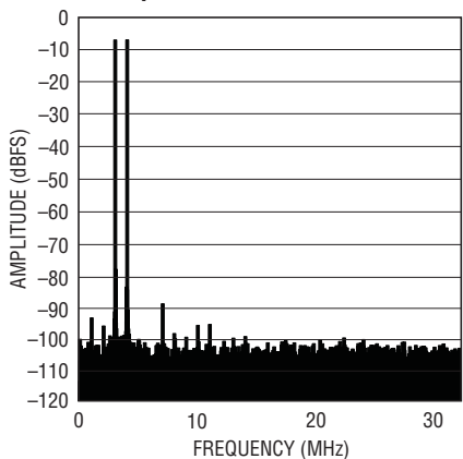
LTC2172-14: 8k Point 2-Tone FFT, f_{IN} = 68\text{MHz} , 69MHz, -1dBFS, 65Mps
