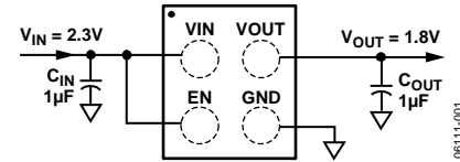
Figure 1. ADP172 with Fixed Output Voltage, 1.8 V
