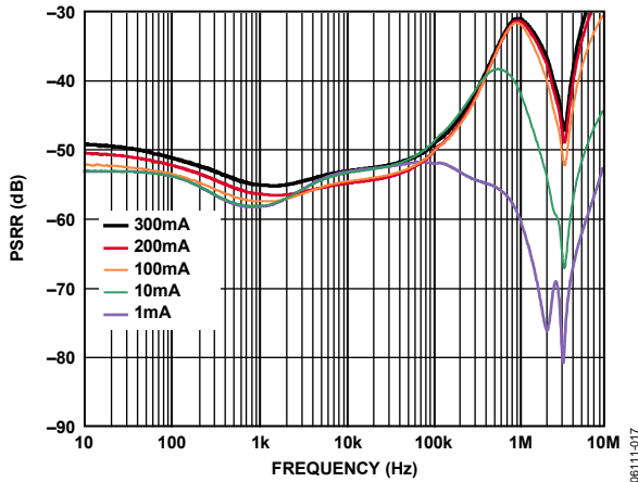
Figure 15. Power Supply Rejection Ratio vs. Frequency, V_{OUT} = 3.0V
