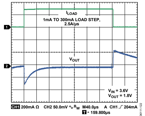
Figure 20. Load Transient Response, C_{IN} and C_{OUT} = 4.7\mu F
