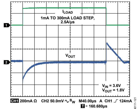
Figure 19. Load Transient Response, C_{IN} and C_{OUT} = 1\mu F
