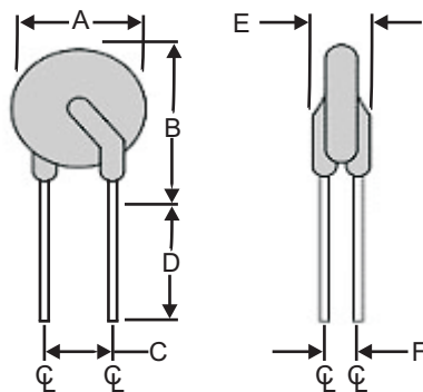
Figure 2 Lead Size: 20AWG Φ 0.81 mm Diameter
