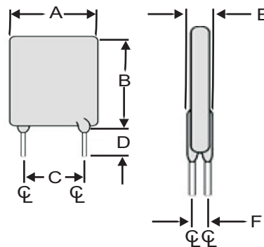
Figure 3 Lead Size: 20AWG Φ 0.81 mm Diameter
