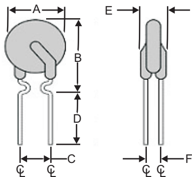
Figure 1 Lead Size: 24AWG Φ 0.51 mm Diameter
