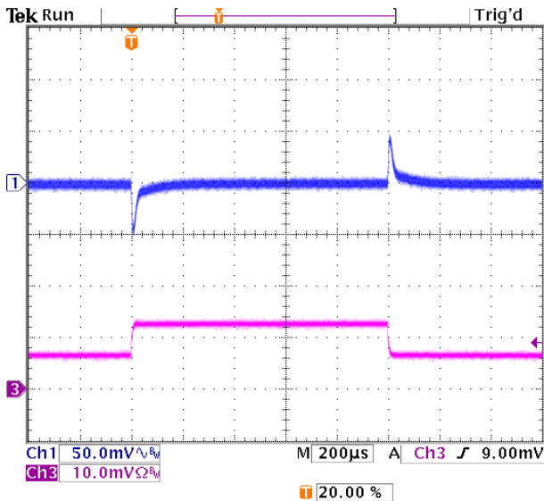
Figure 11. Transient Response to Dynamic Load Change from 40% to 80% of full load ( V_{in}=12V , V_o=3.3Vdc ). Ch3 – Iout. Scale=0.2A/mVΩ
