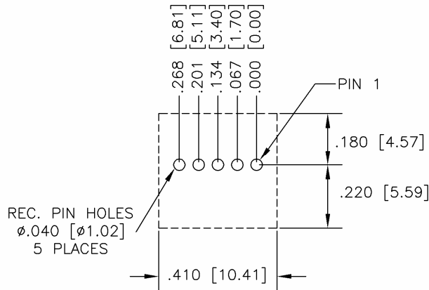
Figure 15. Mechanical Drawing
