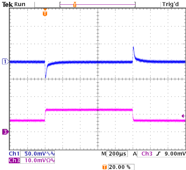
Figure 10. Transient Response to Dynamic Load Change from 40% to 80% of full load ( V_{in}=12V , V_o=2.5Vdc ). Ch3 – Iout. Scale=0.2A/mVΩ
