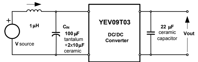
Figure 14. Test Setup For Measuring Input Reflected-Ripple Current And Output Voltage Ripple
