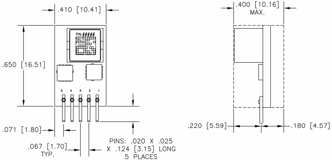
Figure 15. Mechanical Drawing
