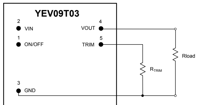
Figure 12. Programming Output Voltage With A Resistor
