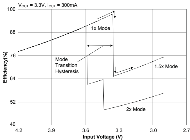
Efficiency — 300mA
