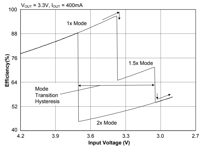
Efficiency — 400mA
