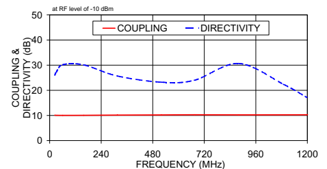
LRDC-10-2W-75 COUPLING & DIRECTIVITY
