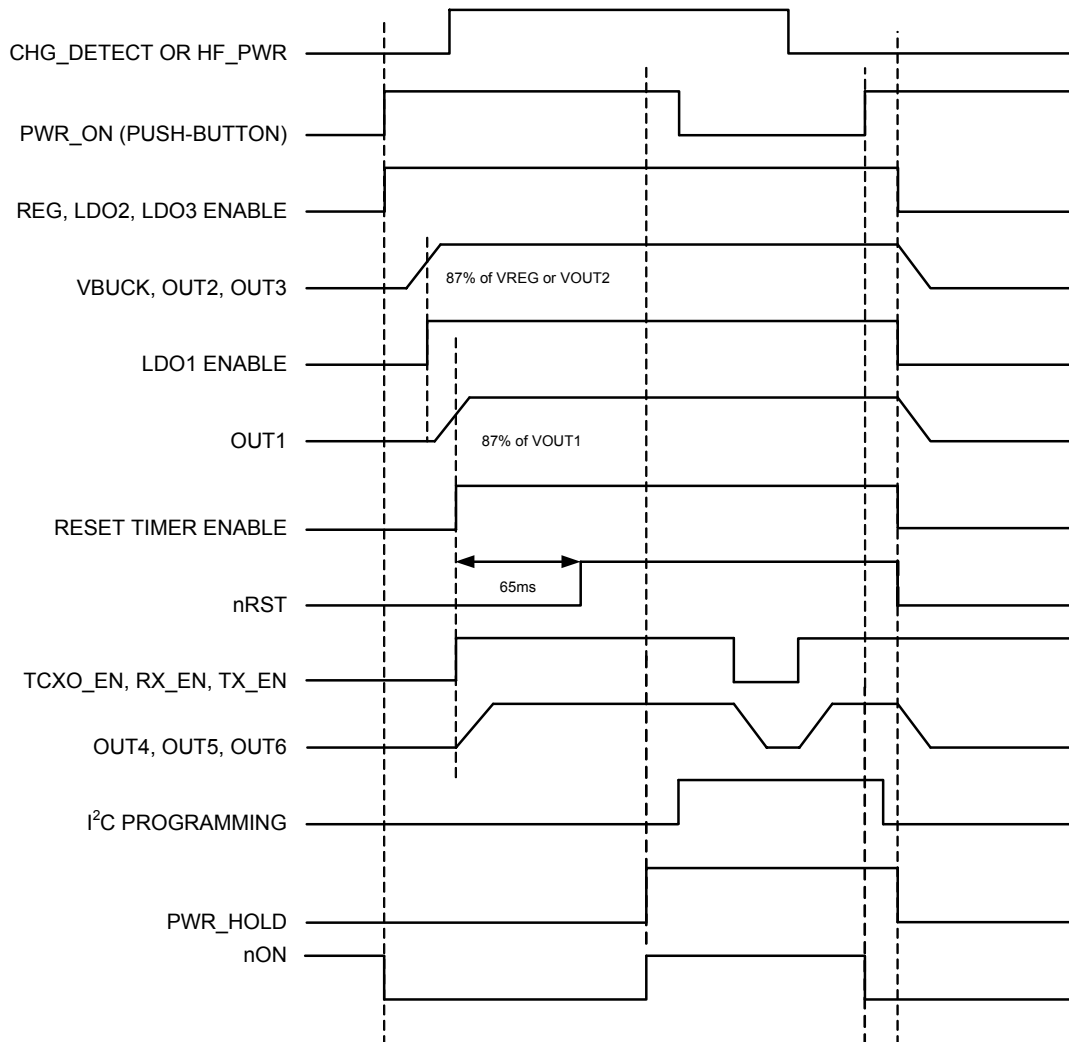
Figure 2: Startup and Shutdown Sequence
