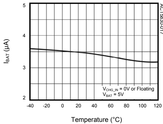
BAT Reverse Leakage Current vs. Temperature
