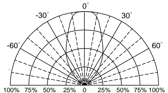
Fig.6 Directivity Radiation
