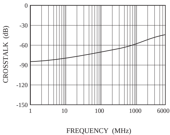
ANALOG CROSSTALK
