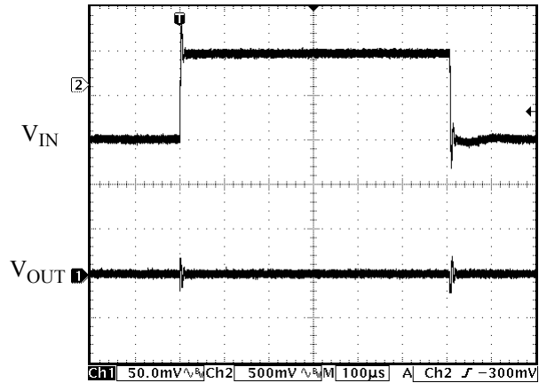
Figure 33. Line Transient
