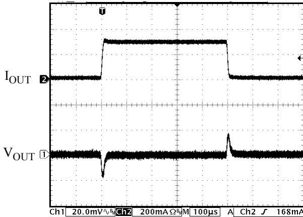
Figure 32. Load Transient
