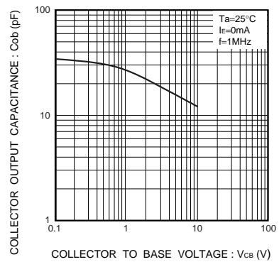
Fig.7 Collector output capacitance vs. collector-base voltage
