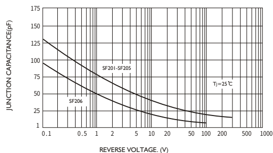
FIG.6-TYPICAL JUNCTION CAPACITANCE
