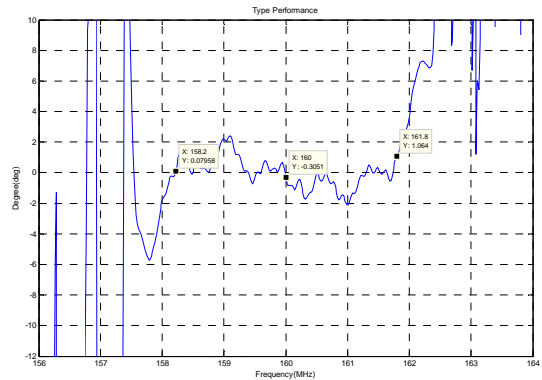
Phase Linearity(f0±1.8MHz)
