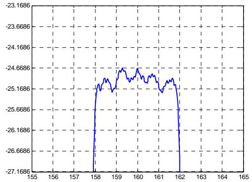
Passband Respond
