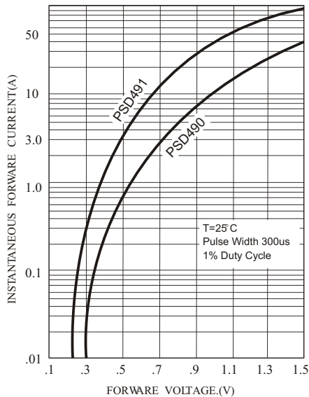
FIG.1 Typical Forward Characteristics
