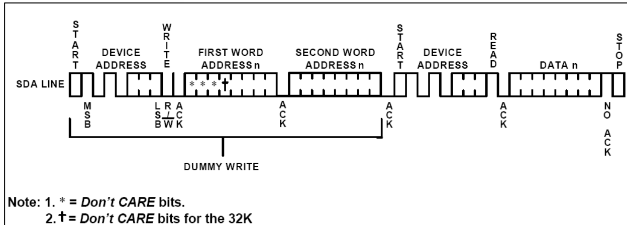
Figure 11 · Random Read
