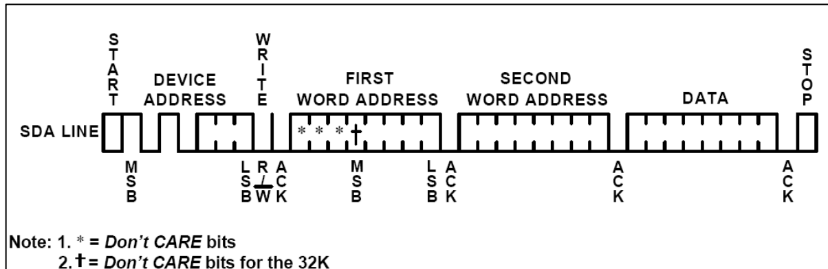
Figure 8 · Byte Write
