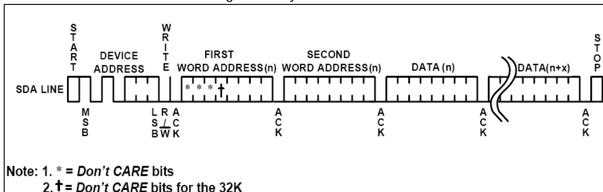
Figure 9 · Page Write
