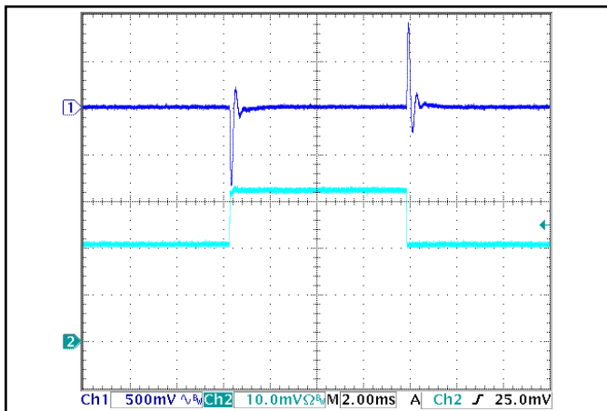
Figure 15: Output voltage response to step-change in load current (50%-75%-50% of I out (max); di/dt = 0.1A/μs). Load cap: 10μF, 100 mΩ ESR tantalum cap and 1μF ceramic cap. Ch 1: V out (500mV/div), Ch 2: I out (2A/div).
