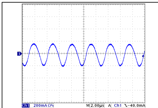
Figure 18: Input Terminal Ripple Current, I C , at full rated output current and nominal input voltage with 10μH source impedance and 47μF electrolytic capacitor (200 mA/div). See Figure 17.
