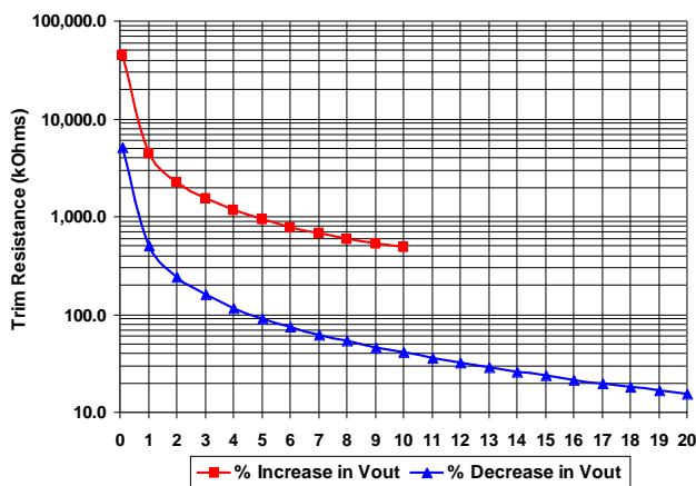
Figure C: Trim Graph
