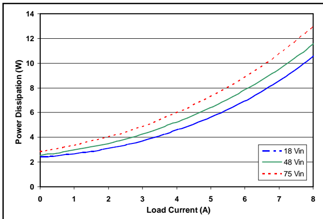
Figure 3: Power dissipation at nominal output voltage vs. load current for 18V, 48V and 75V input at 25°C.
