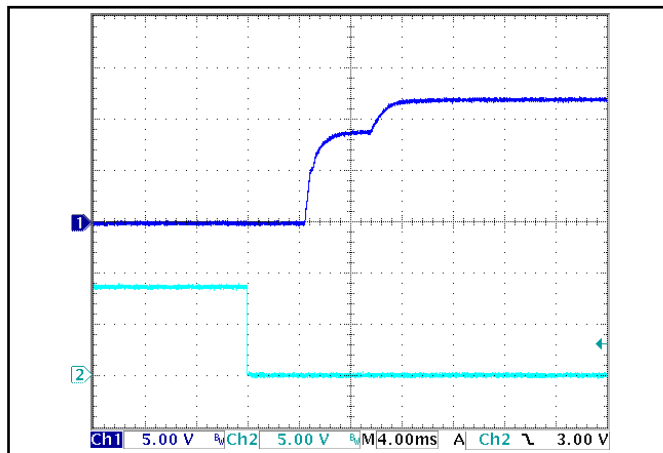
Figure 14: Turn-on transient at zero load (4 ms/div). Ch 1: V out (5V/div). Ch 2: ON/OFF input (5V/div).
