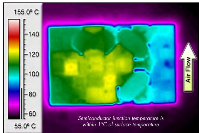
Figure 6: Thermal plot of converter at 8.33 amp load current with 55°C air flowing at the rate of 200 LFM. Air is flowing across the converter sideways from pin 3 to pin 1 (24V input).
