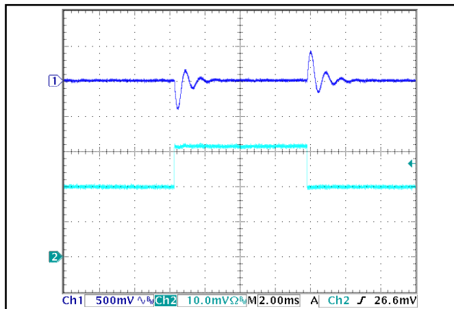
Figure 16: Output voltage response to step-change in load current (50%-75%-50% of I out (max); di/dt = 5A/μs). Load cap: 470μF, 30 mΩ ESR tantalum cap and 1μF ceramic cap. Ch 1: V out (500mV/div), Ch 2: I out (2A/div).
