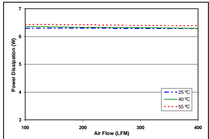
Figure 4: Power dissipation at nominal output voltage and 60% rated power vs. airflow rate for ambient air temperatures of 25°C, 40°C, and 55°C (nominal input voltage, 48V input).
