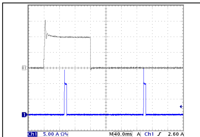
Figure 22: Load current (5A/div) as a function of time when the converter attempts to turn on into a 10\ \text{m}\Omega short circuit. Top trace (40ms/div) is an expansion of the on-time portion of the bottom trace.
