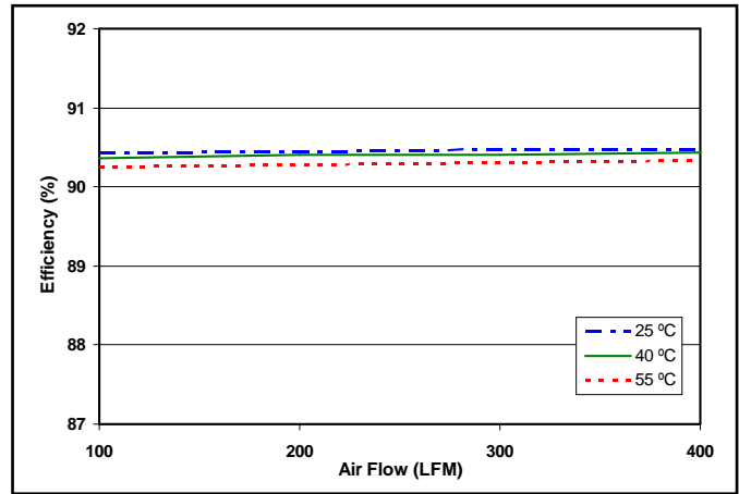
Figure 2: Efficiency at nominal output voltage and 60% rated power vs. airflow rate for ambient air temperatures of 25°C, 40°C, and 55°C (nominal input voltage, 48V input).
