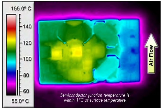
Figure 8: Thermal plot of converter at 8.1 amp load current with 55°C air flowing at the rate of 200 LFM. Air is flowing across the converter sideways from pin 3 to pin 1 (48V input).
