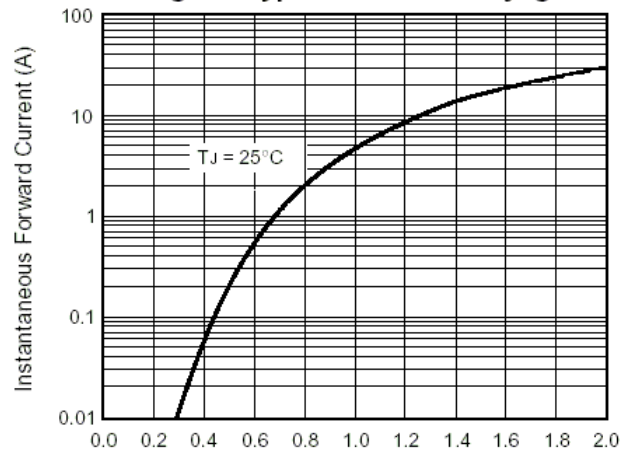
Fig. 4 – Typical Forward Voltyage
