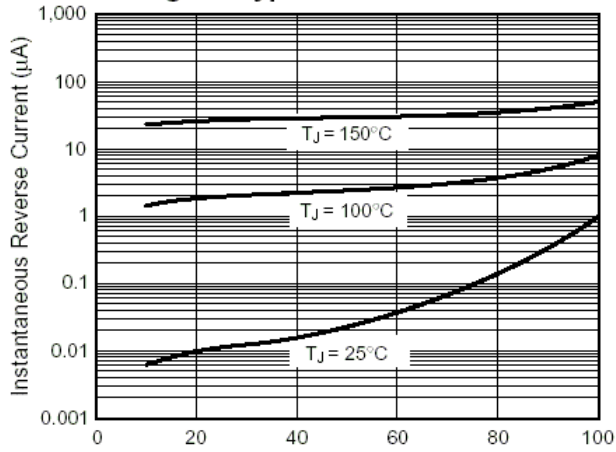
Fig. 3 – Typical Reverse Current
