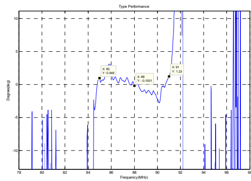
Phase Linearity (f0±3MHz)
