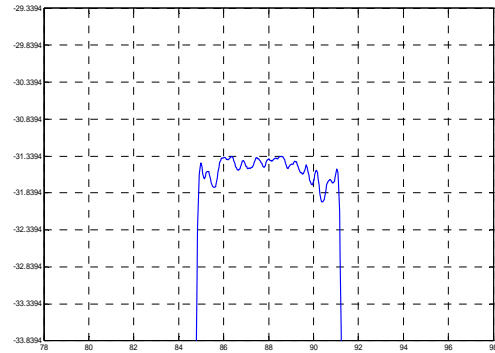
Passband Response
