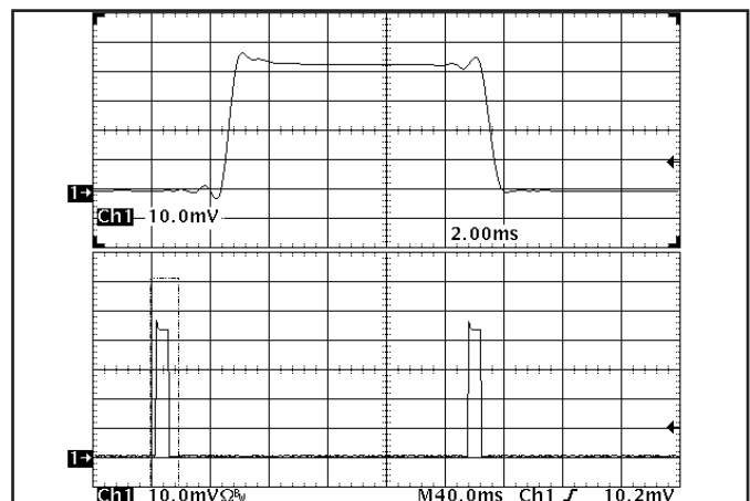
Figure 18: Load current ( 20\text{A}/\text{div} ) as a function of time when the converter attempts to turn on into a 1\ \text{m}\Omega short circuit. Top trace ( 2\text{ms}/\text{div} ) is an expansion of the on-time portion of the bottom trace.
