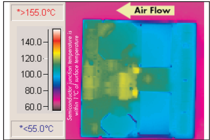
Figure 8: Thermal plot of converter at 55 amp load current with 55°C air flowing at the rate of 200 LFM. Air is flowing across the converter from output to input (nominal input voltage).
