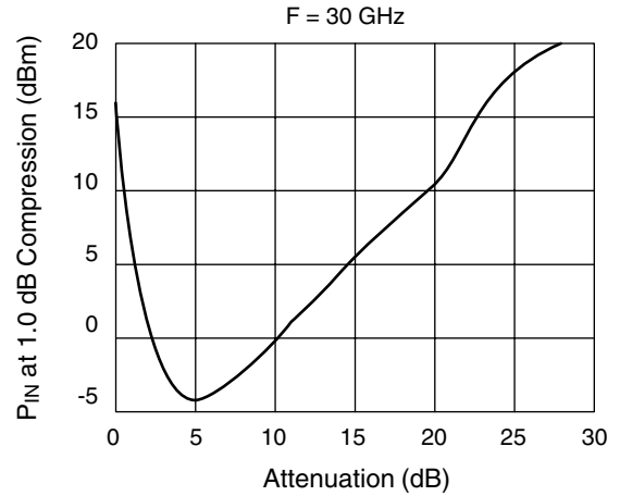
Attenuation vs. 1.0 dB Compression Point
